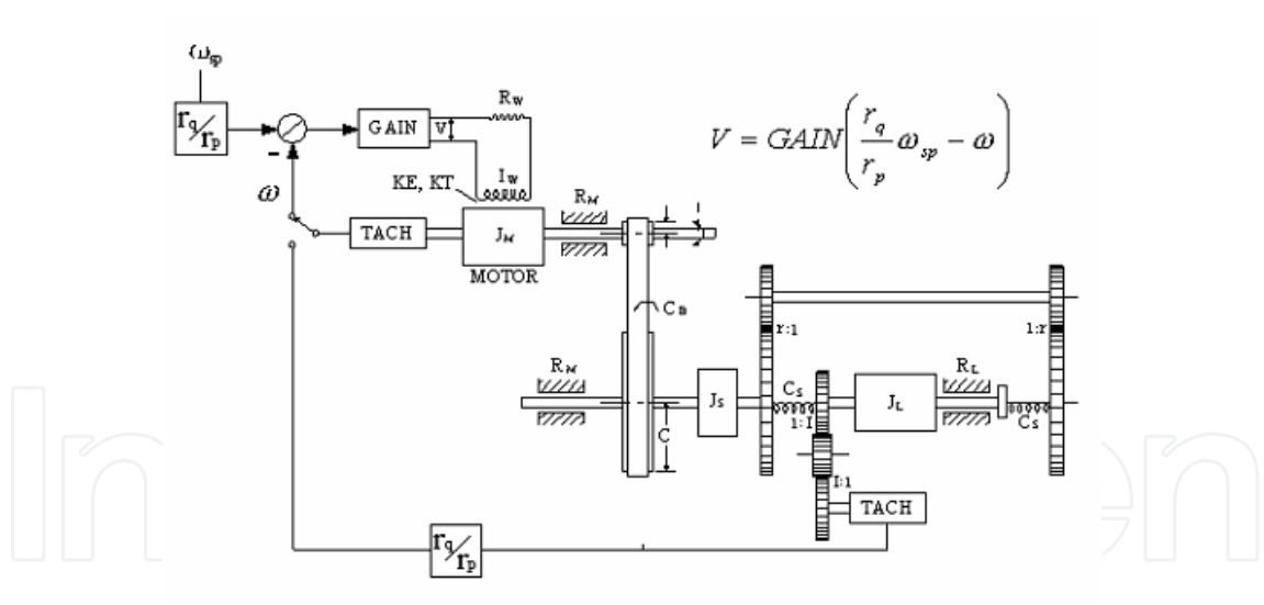
Figure 7. Schematic of the typewriter drive system
