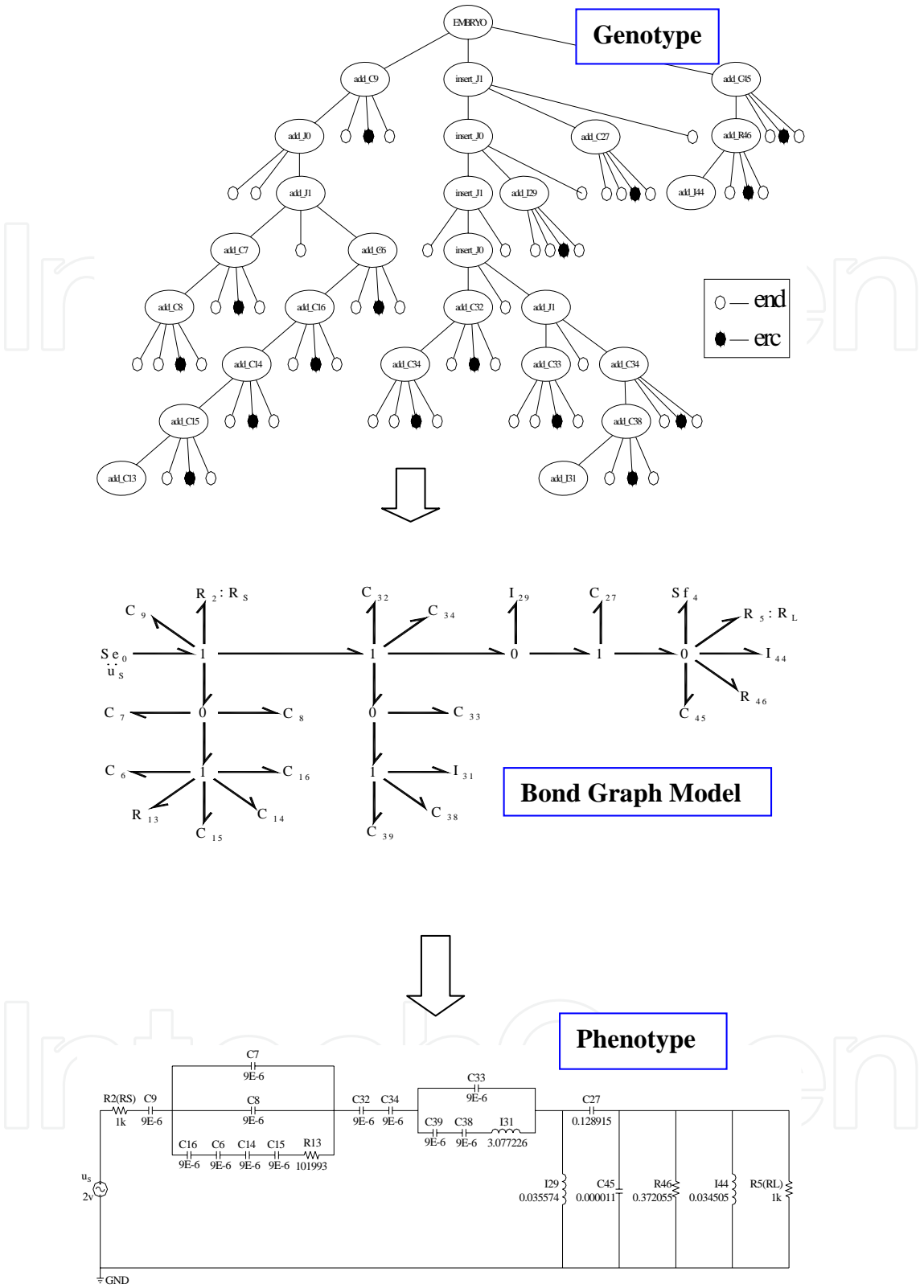
Figure 3. Example of Genotype-Phenotype Mapping in the Electrical Circuit Domain
