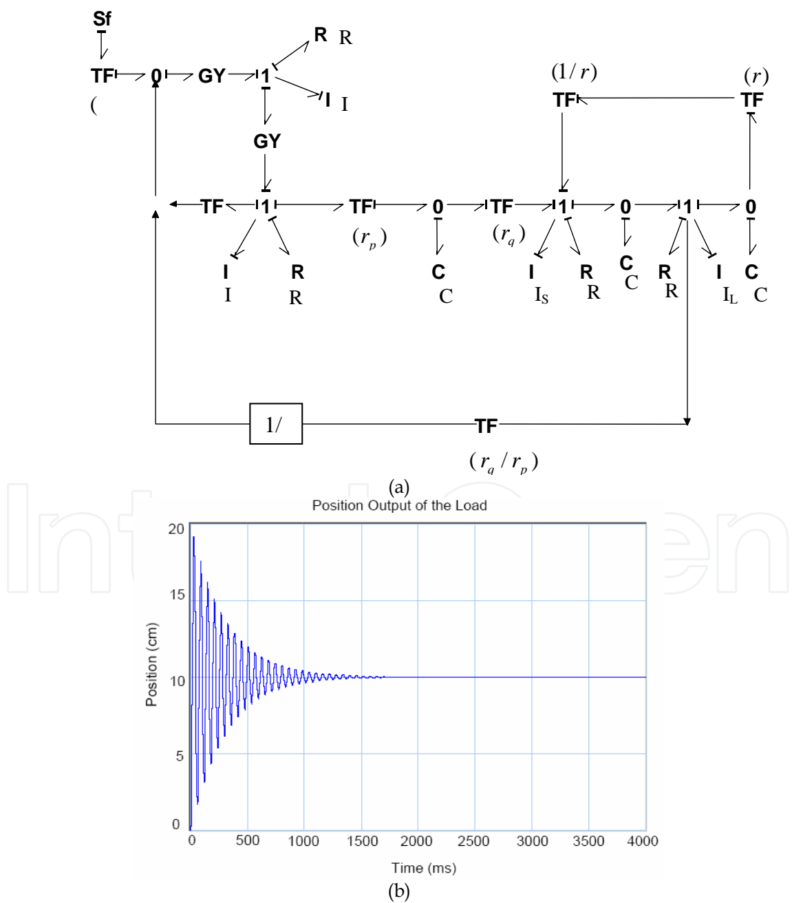
Figure 8. a) Bond graph model b) Positional vibration of the load
