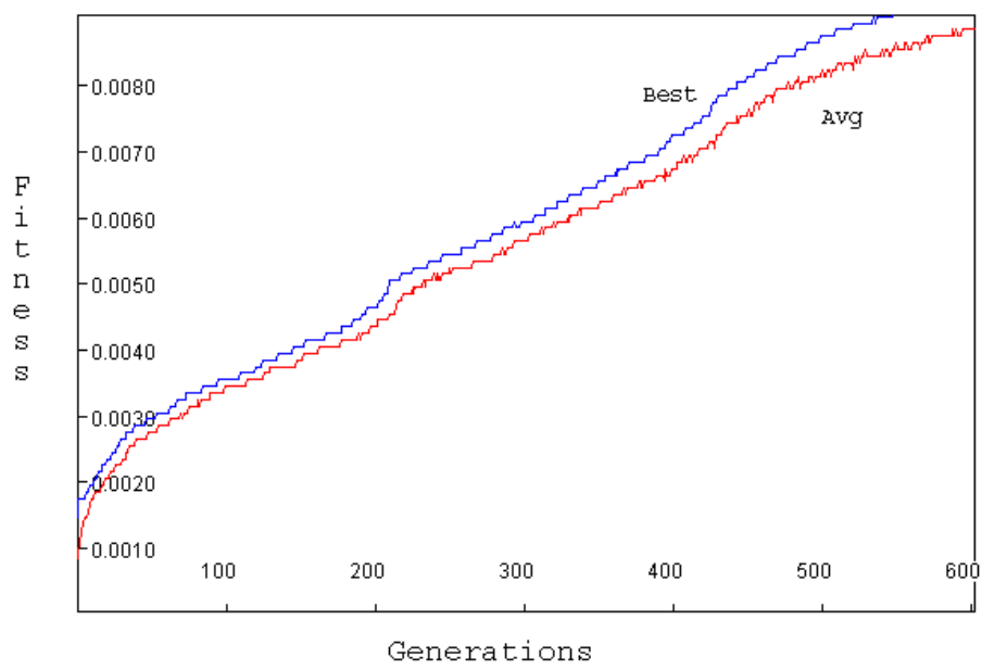
Fig. 10. Fitness progress for clothing texture run.
