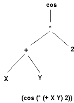
Fig. 2. Example tree and corresponding expression
