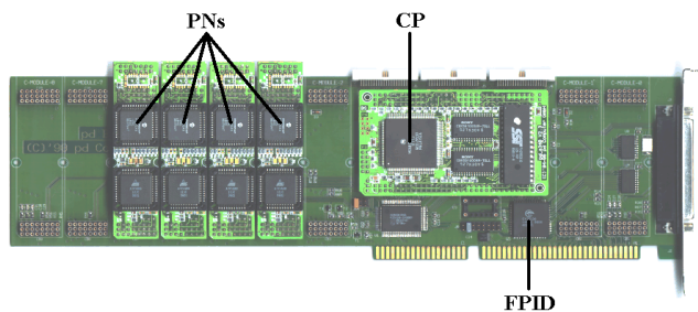
Figure 1: Layout of the carrier board
