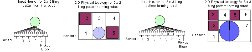
Fig. 4. Input layer neuron and physical topology for the 2 \times 2 (left) and 3 \times 3 (right) tiling pattern forming robots.
