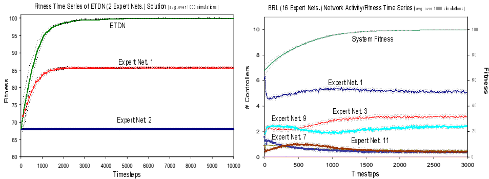
Fig. 6. (left) Fitness of individual expert networks and the entire control system (ETDN, 2 expert nets.) averaged over 1000 simulations. (right) Expert Network activity and overall system fitness for a BRL (with 16 expert networks).
