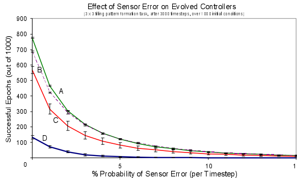
Fig. 7. Effect of sensor error on evolved controllers (population best at Generation 200) for the 3 \times 3 tiling pattern formation task ( 16 \times 16 world, 11 robots, 36 blocks, after 3000 timesteps) averaged over 1000 simulations. (A) BRL (16 Expert Nets, Modular), (B) ETDN (2 Expert Nets), (C) Non-Emergent Net. (Modular), (D) Non-Emergent Net (Sigmoid).
