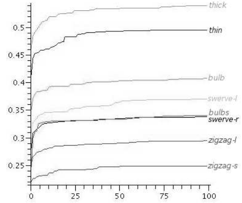
Figure 3: Plot of the mean of maximum fitness for the sets of runs in each environment: fitness ( y -axis) versus generation ( x -axis).
