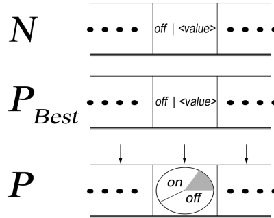
Figure 1: Pheromone Update in PSO/ACO2
