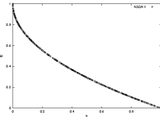
Non-dominated solutions found for ZDT1.
