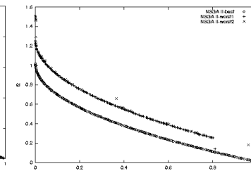
Non-dominated solutions found for ZDT4.
