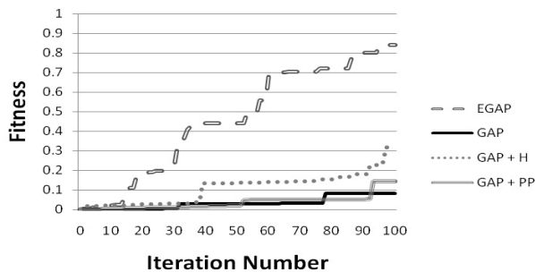
Figure 6. Plot of the mean of the best fitness on quartic symbolic regression problem during the 100 iterations
