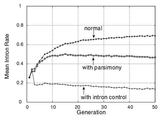
(b) Intron Rate vs. Generations
