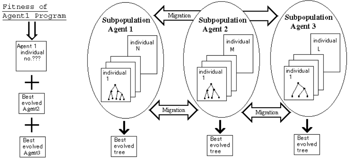
Figure 2: Co-evolutionary Breeding for Multi-Agent Learning
