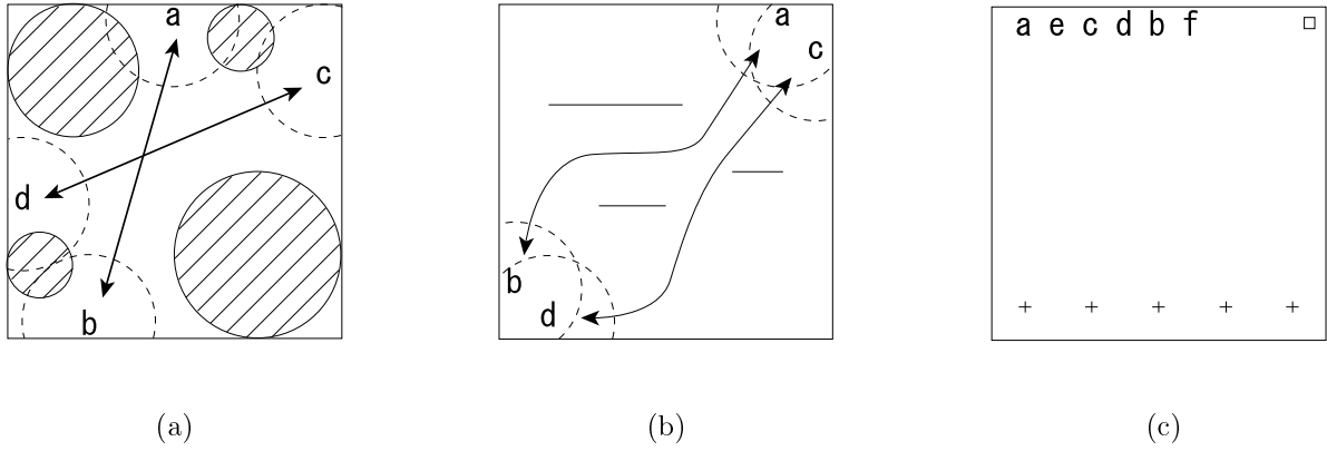
Figure 1: Training Maps for Robot Tasks
