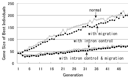
(a) Program Sizes.
