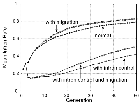
(b) Intron Rate vs. Generations
