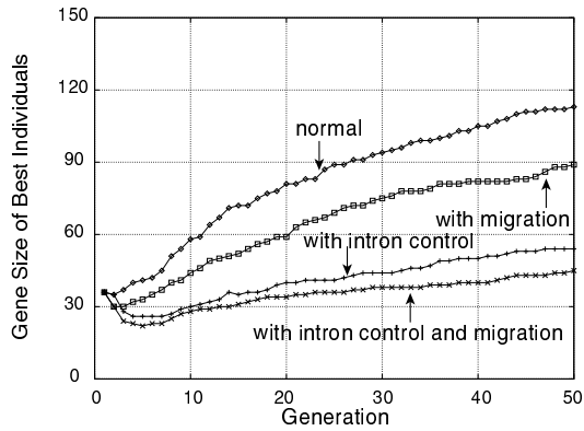
(c) Program Size vs. Generations
