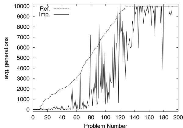
Figure 1 : Average Generation
