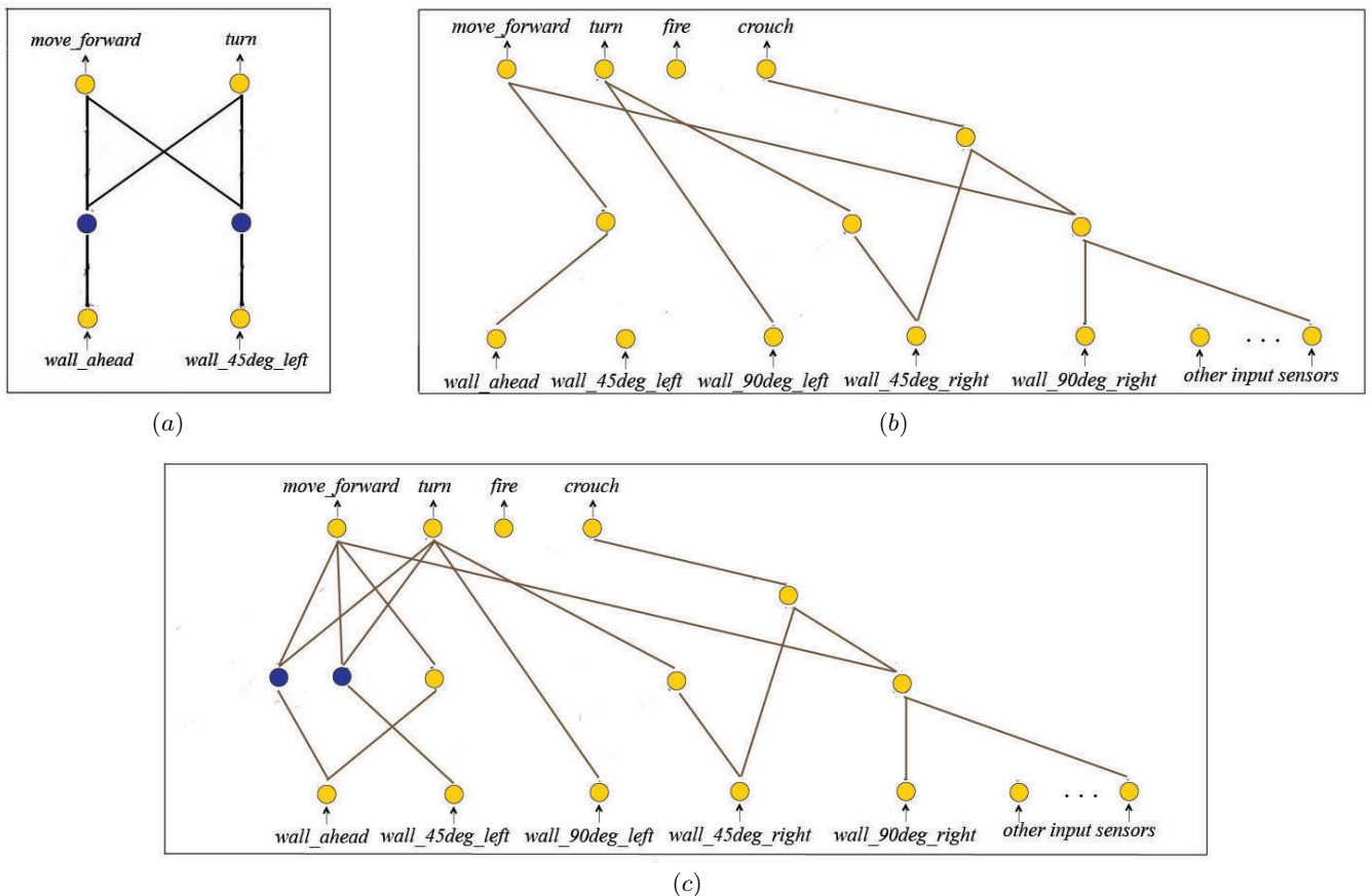
Figure 5. Incorporating advice into neural networks in NERO. (a) The network structure that implements the advice in Figure 3. The thresholds and weights of each hidden unit is set so that they implement the two rules. (b) A network controlling the agents before the advice. (c) The advice is added by connecting the hidden nodes of the advice structure to the appropriate inputs and outputs.
