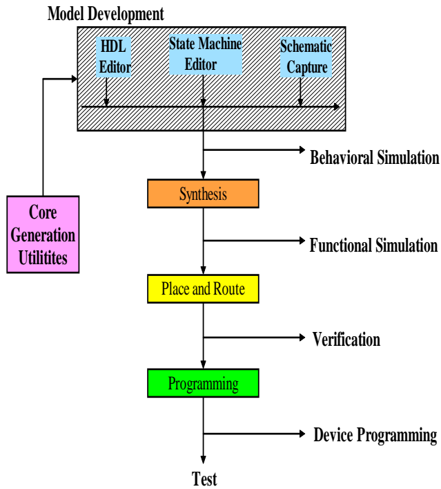
Figure 6. FPGA Design Flow
