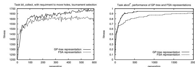
Figure 1: Performance of the FSA and GP-tree representations on symbolic tasks without sufficient repetitive interactions. The GP representation outperforms the FSA representation. Average of best indiv. in each generation from 10+ /23+ runs.
