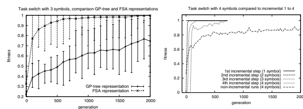
Figure 2: Average of the best fitness from 10+ runs on a symbolic task with repetitive FSA representation. FSA representation outperforms the GP-tree representation (left). Incremental evolution speeds up evolution and increases evolvability (right).
