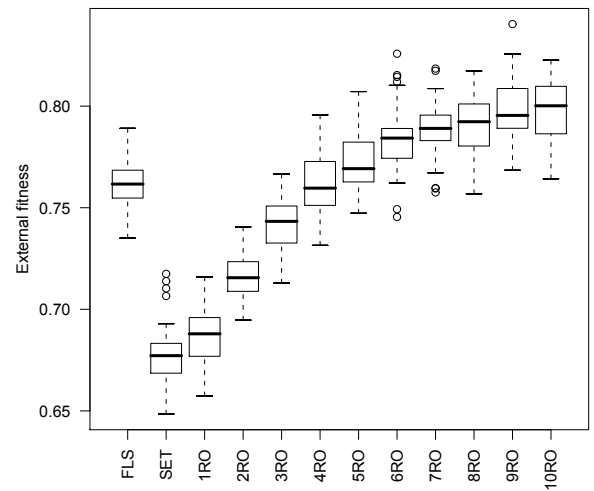
Figure 14: Rastrigin with 40% noise
