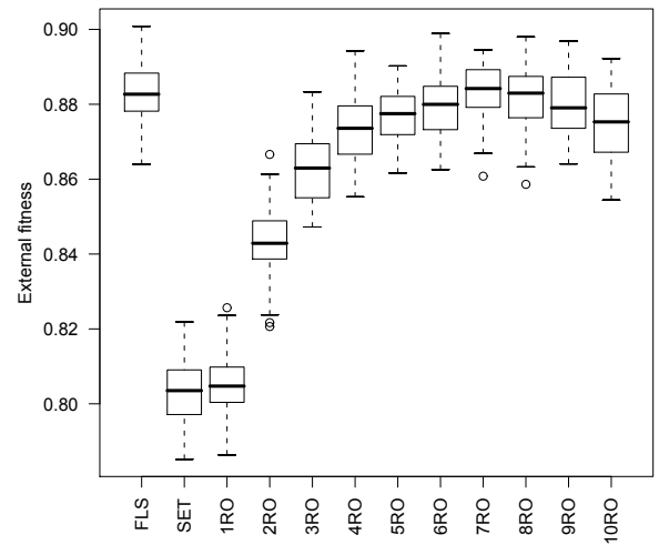
Figure 13: Rastrigin with 30% noise
