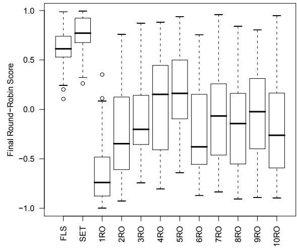
Figure 6: Nim with 0% noise
