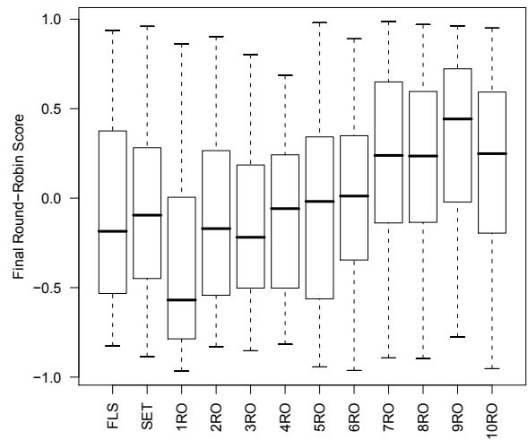
Figure 8: Nim with 40% noise
