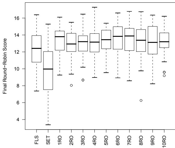
Figure 5: Tic Tac Toe with 40% noise
