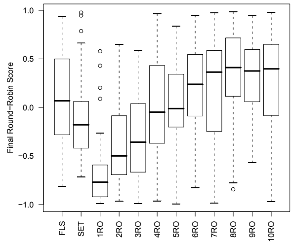
Figure 7: Nim with 30% noise
