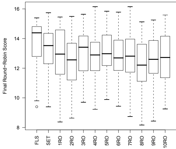
Figure 3: Tic Tac Toe with 0% noise
