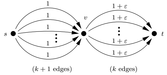
Figure 3. Graph H_k
