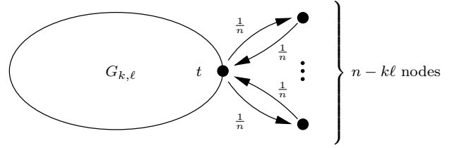
Figure 2. Graph G'_{k, \ell}
