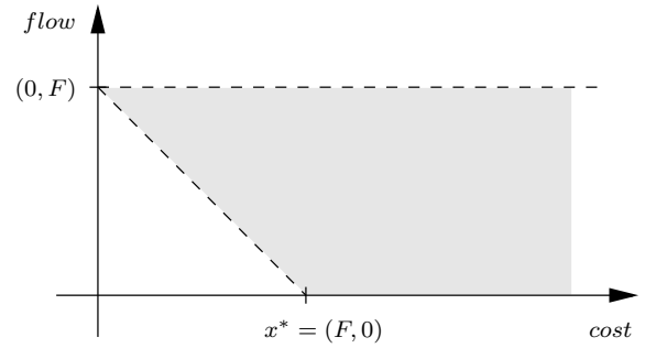
Figure 5. Objective space of the fitness function f(x) = (cost(x), flow(x))
