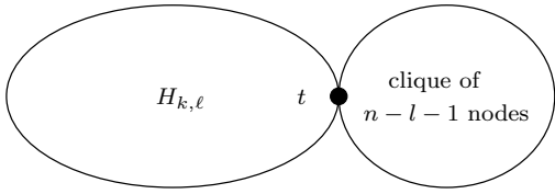
Figure 4. Graph H'_{k,\ell}
