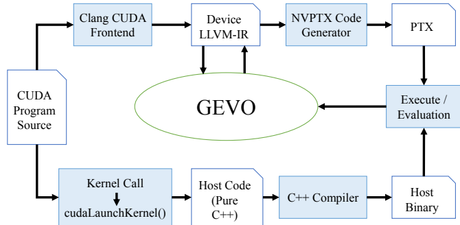
Fig. 1: GEVO in the LLVM/Clang compilation flow.
